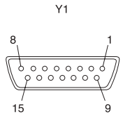
15 Pin D-Type Connector
