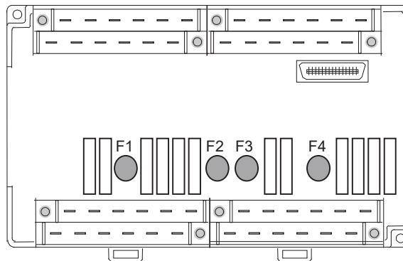
28-Point Micro PLC (IC200UAA007)
