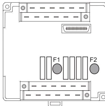
14-Point Micro PLC (IC200UAA003)
