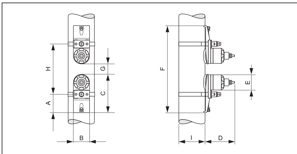
Mounting arrangement for measurement via two traverses
