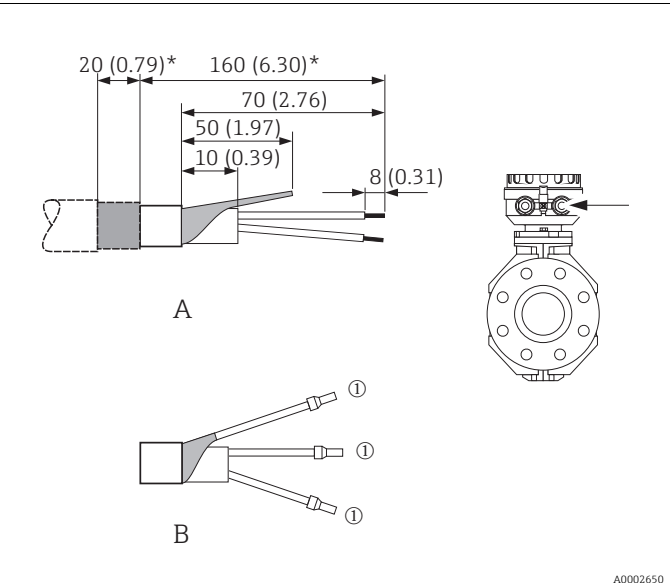
Fig. 35: Engineering unit mm (inch)
