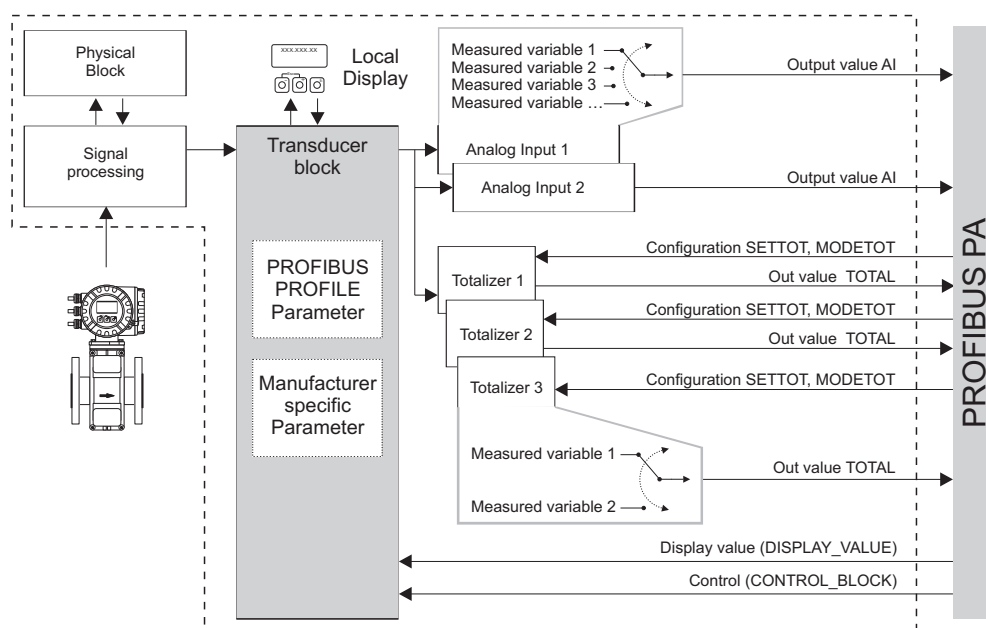
Fig. 72: Block model for Promag 53 PROFIBUS PA Profile 3.0
