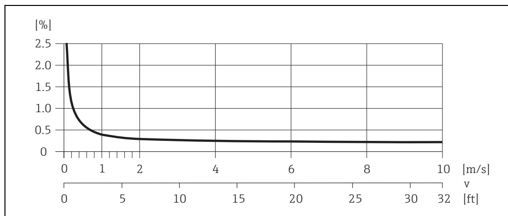
Fig. 82: Max. measured error in % of reading
