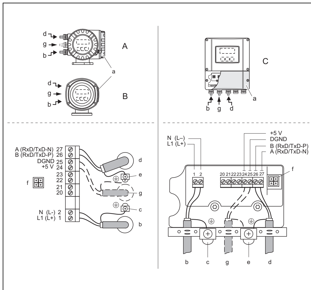
Fig. 41: Connecting the transmitter, cable cross-section: max. 2.5 mm 2 (14 AWG)
