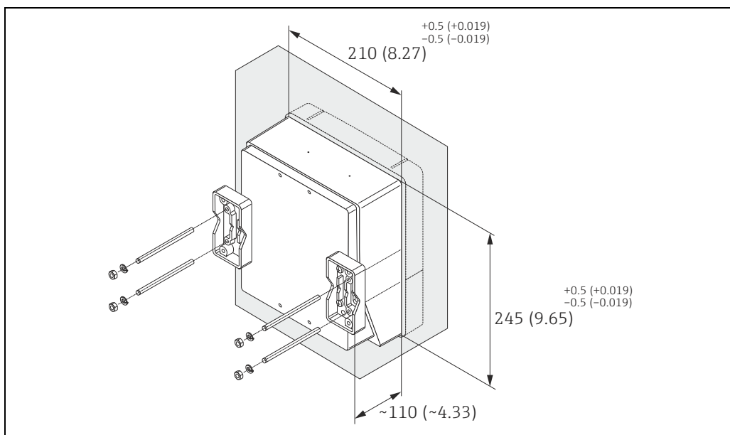
Fig. 28: Panel mounting (wall-mount housing). Engineering unit mm (inch)
