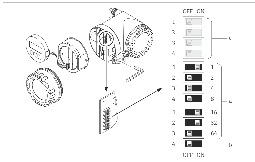
Fig. 62: Addressing with the aid of miniature switches on the I/O board
