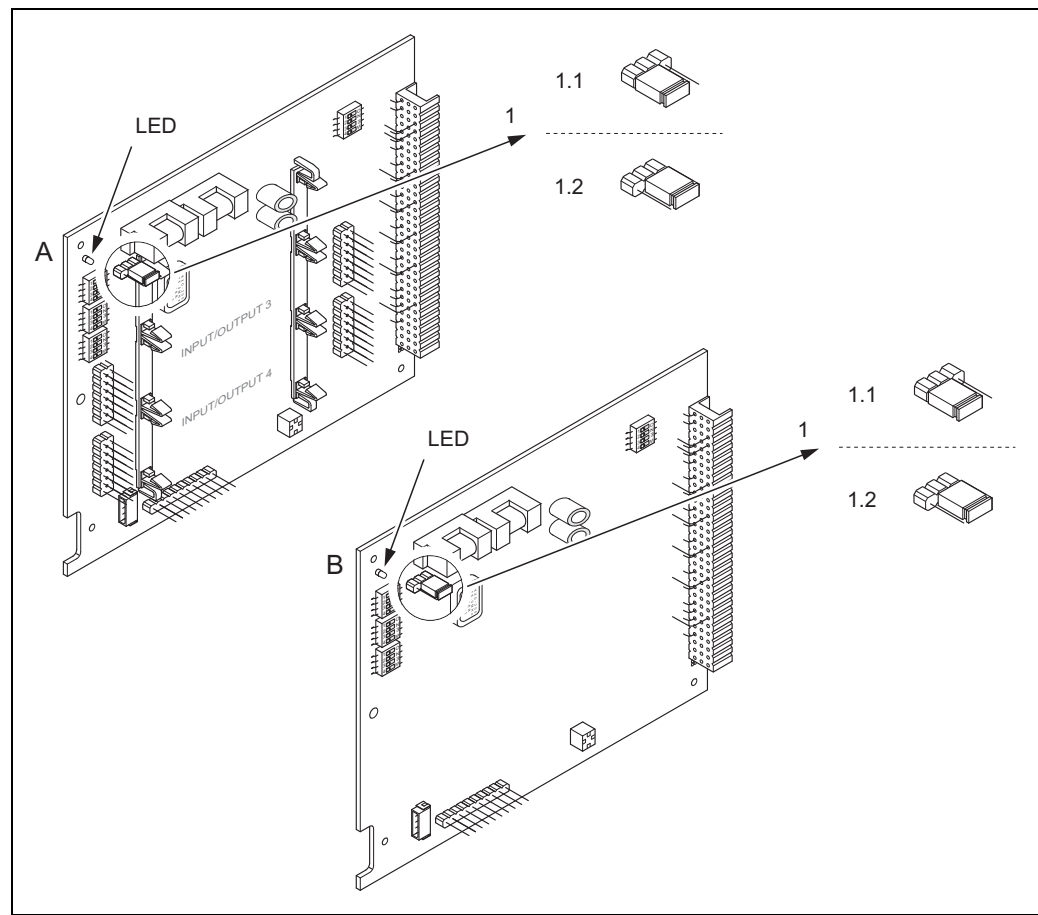
Fig. 56: Switching write protection on and off with the aid of a jumper on the I/O board
