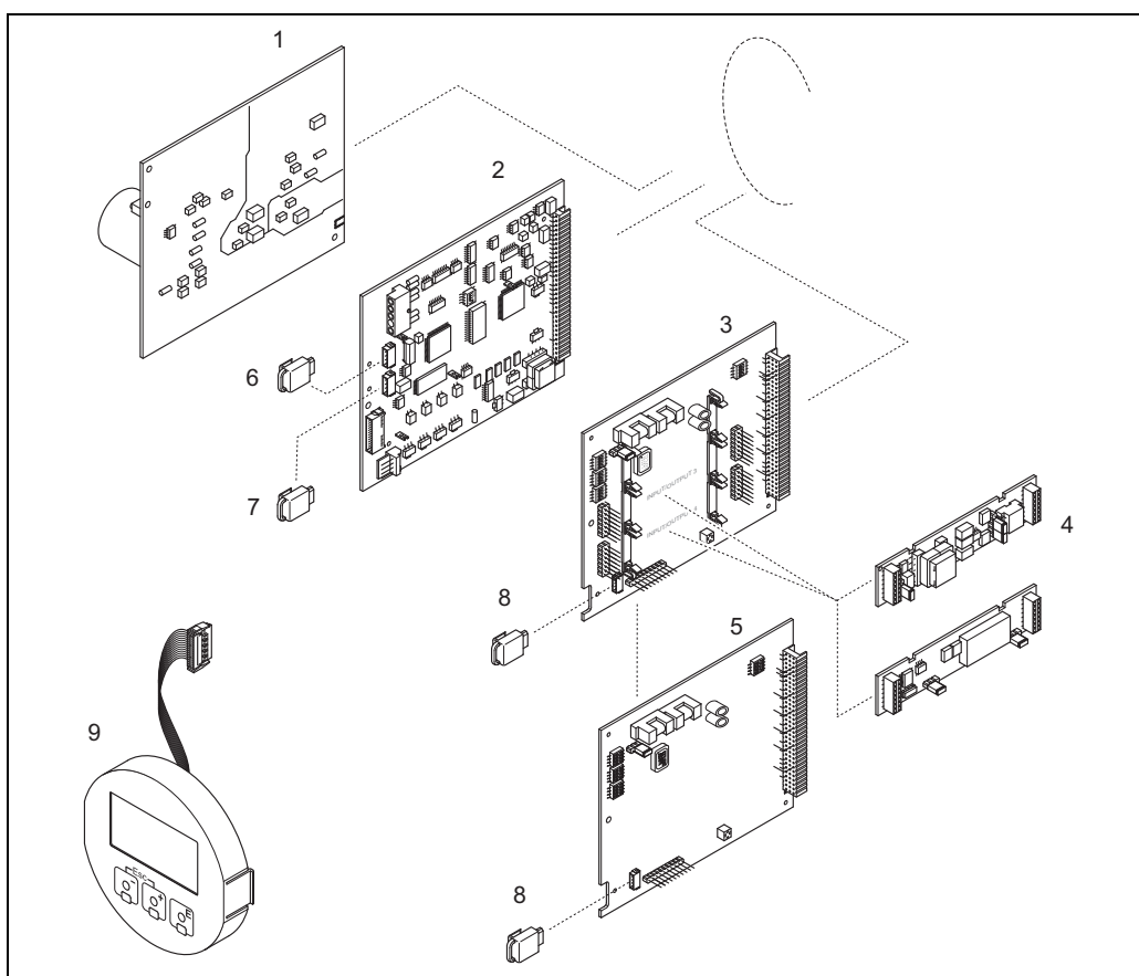
Fig. 76: Spare parts for PROFIBUS DP transmitters (field and wall-mount housing)
