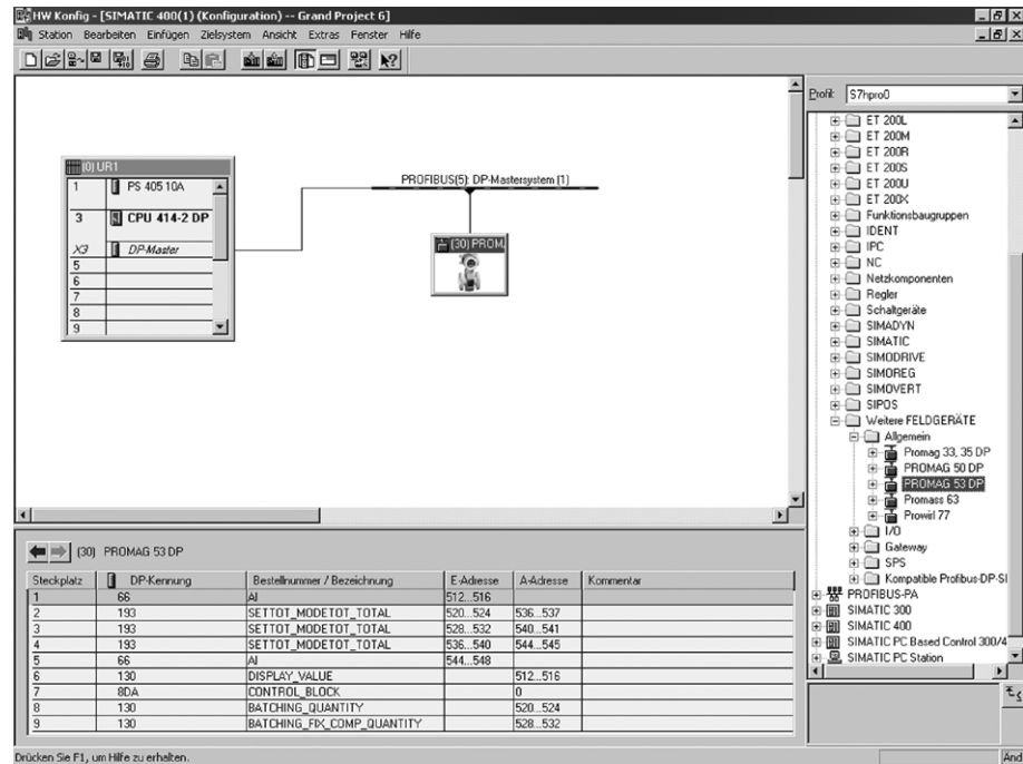
Fig. 70: Complete configuration using the Promag 53 GSD file (complete device functionality)
