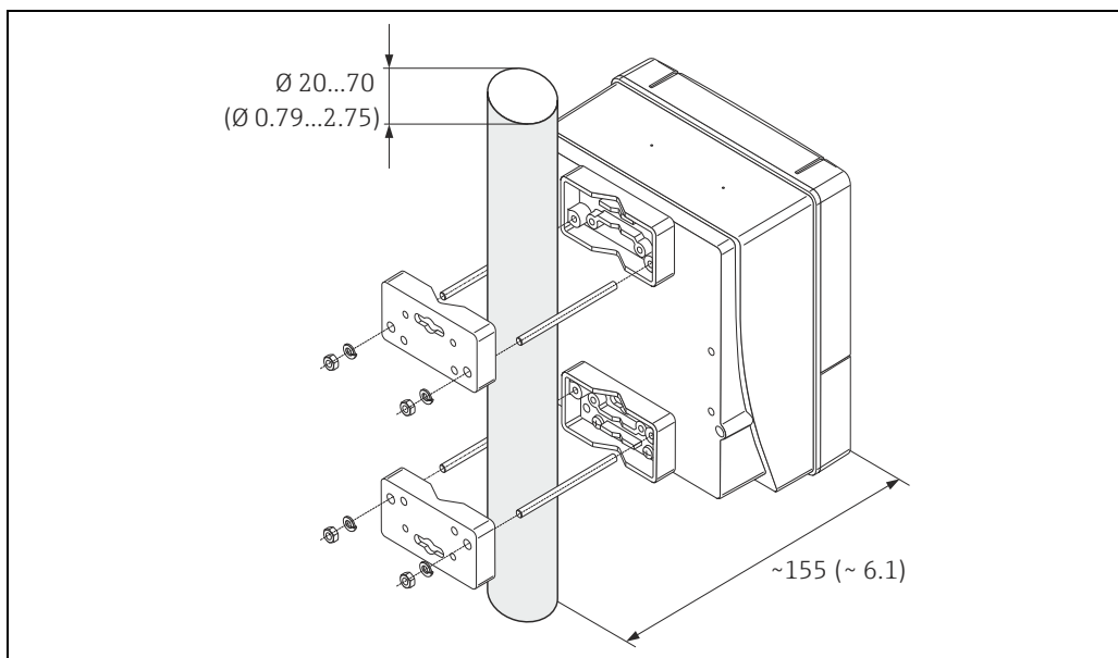
Fig. 29: Pipe mounting (wall-mount housing). Engineering unit mm (inch)
