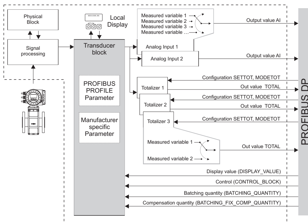
Fig. 69: Block model for Promag 53 PROFIBUS DP Profile 3.0
