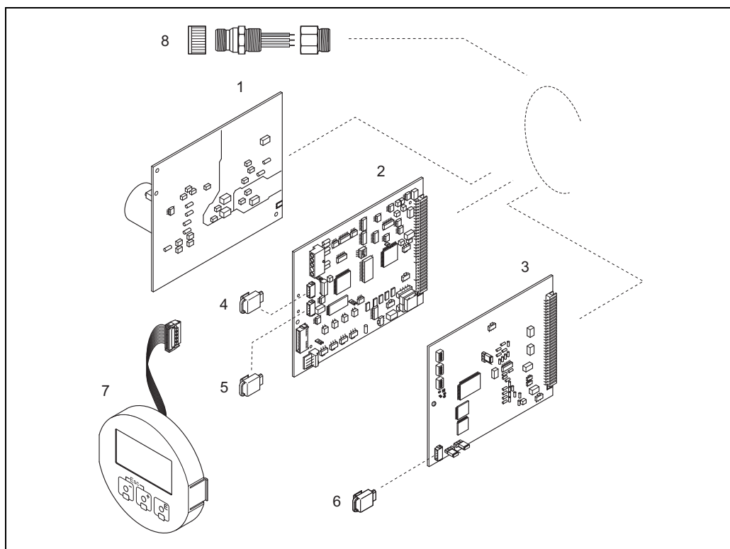
Fig. 77: Spare parts for PROFIBUS PA transmitters (field and wall-mount housing)
