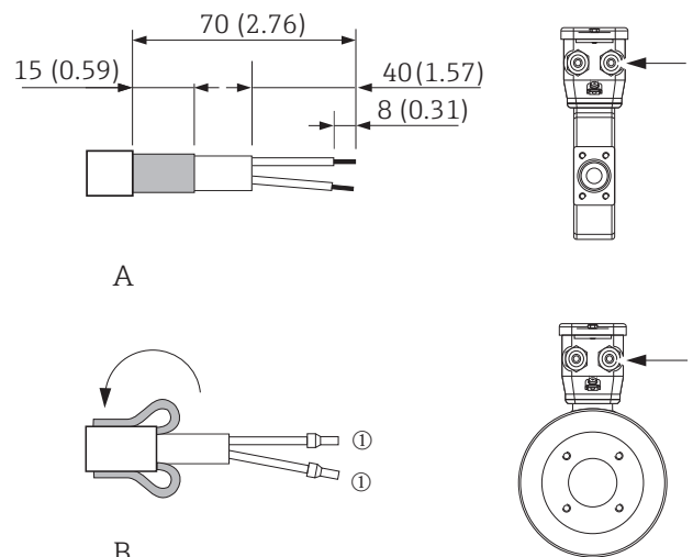
Fig. 39: Engineering unit mm (inch)
