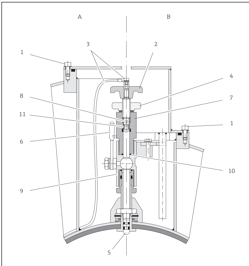
Fig. 81: Apparatus for replacing exchangeable measuring electrodes
