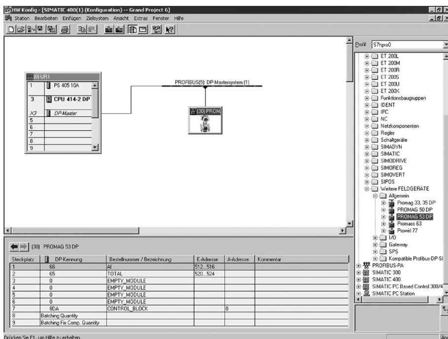
Fig. 71: In this example, modules that are not needed are replaced by the module EMPTY_MODULE. The Promag 53 GSD file is used (manufacturer-specific GSD file, complete device functionality)
