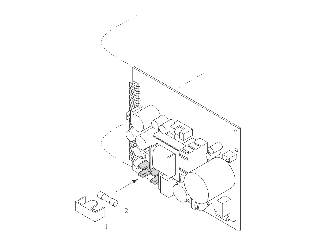
Fig. 80: Replacing the device fuse on the power unit board
