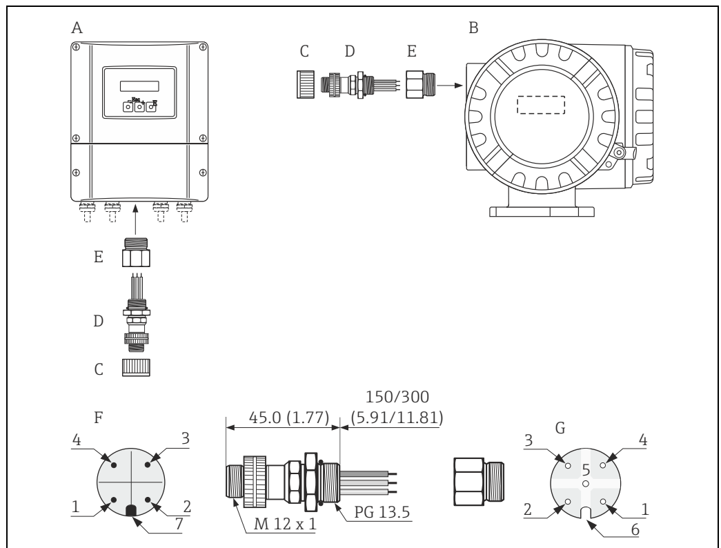
Fig. 44: Connectors for connecting to the PROFIBUS PA. Engineering unit mm (inch)
