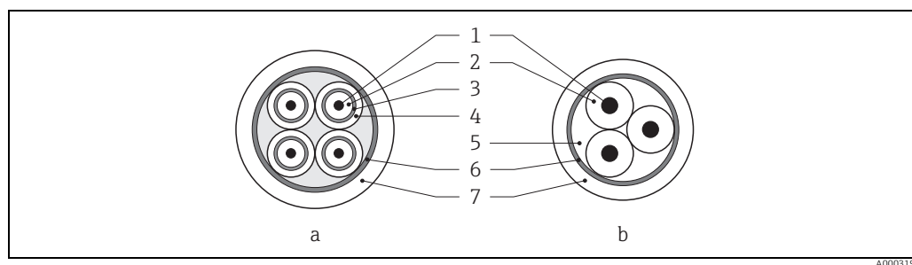
Fig. 40: Cable cross-section
