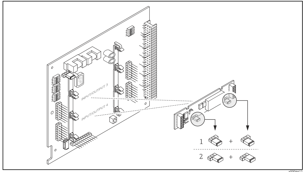
Fig. 60: Configuring relay contacts (NC/NO) on the convertible I/O board (submodule) with the help of jumpers.
