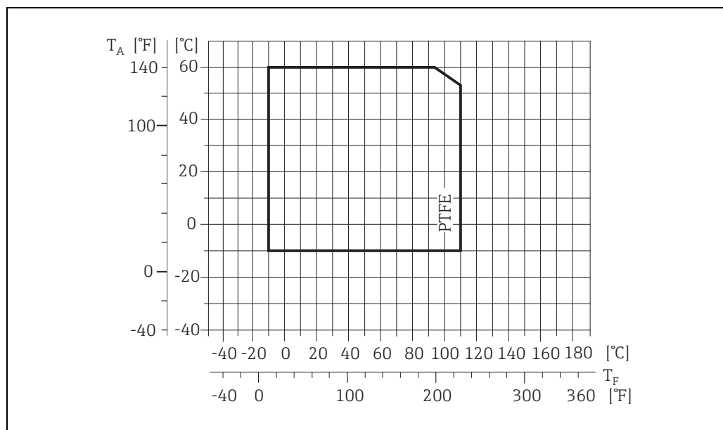
Fig. 83: Compact and remote version ( T_A = Ambient temperature, T_F = Fluid temperature)
