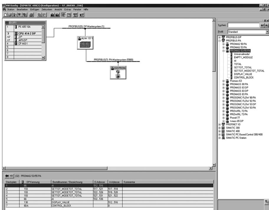
Fig. 73: Complete configuration using the Promag 53 GSD file (complete device functionality)
