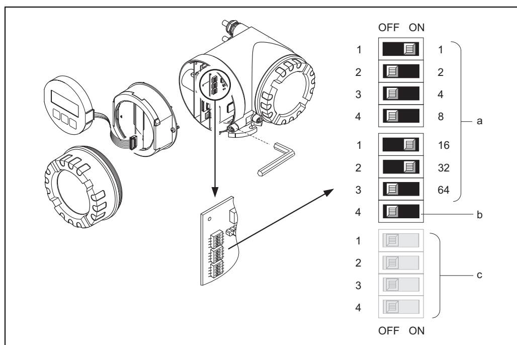
Fig. 57: Addressing with the aid of miniature switches on the I/O board
