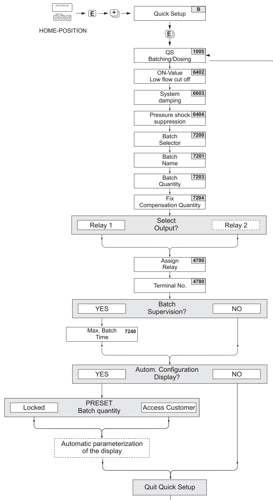
Fig. 66: Quick Setup "Batching". Recommended settings see next page.
