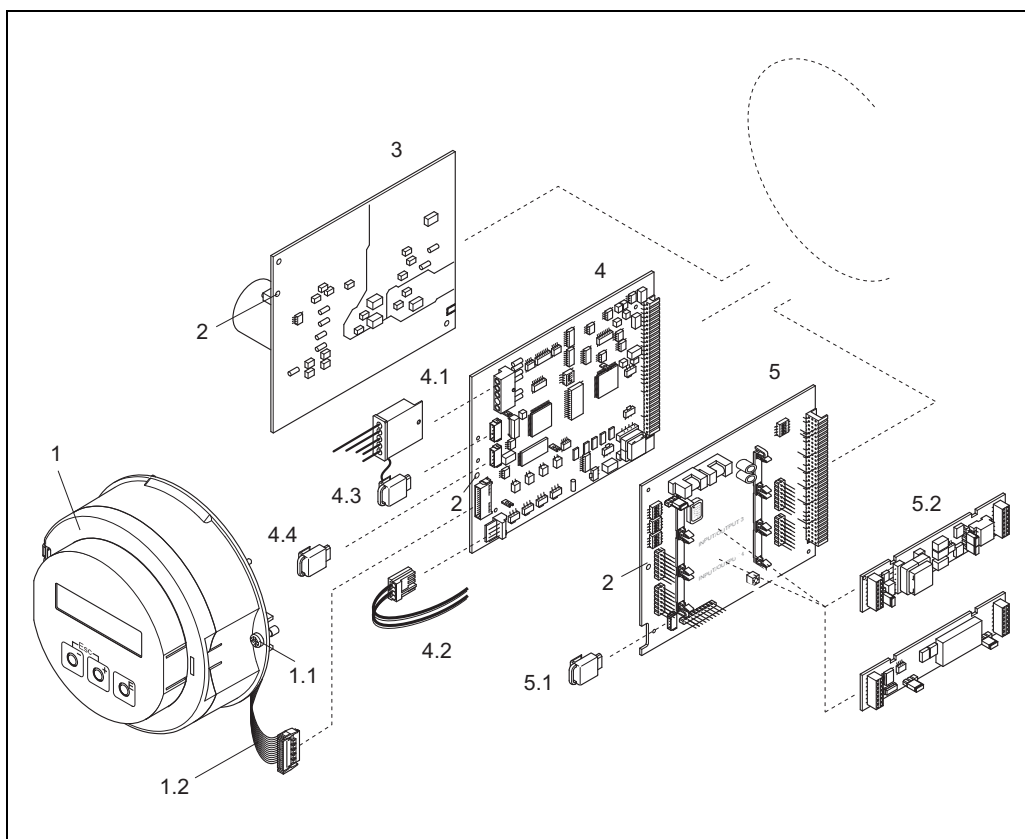
Fig. 78: Field housing: removing and installing printed circuit boards
