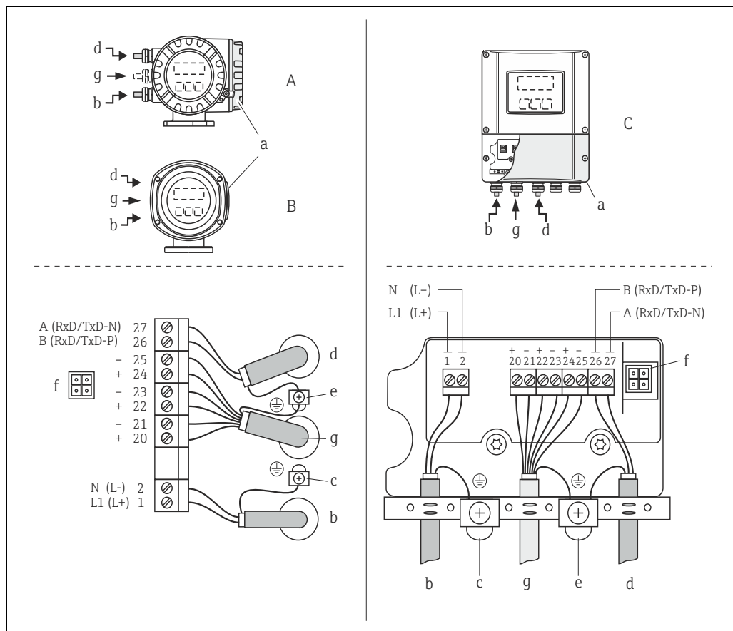
Fig. 42: Connecting the transmitter, cable cross-section: max. 2.5 mm 2 (14 AWG)
