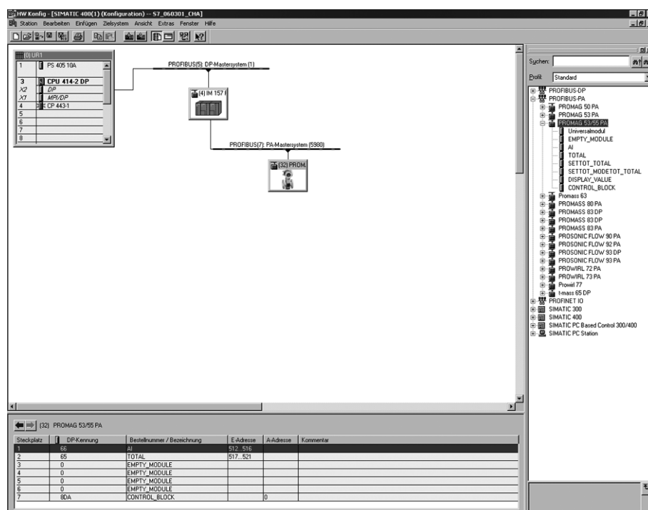
Fig. 74: In this example, modules that are not needed are replaced by the module EMPTY_MODULE . The Promag 53 GSD file is used (manufacturer-specific GSD file, complete device functionality)
