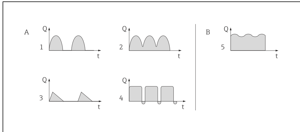
Fig. 64: Flow characteristics of various types of pump
