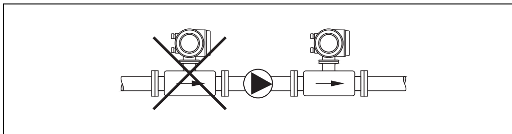
Fig. 7: Installing pumps
