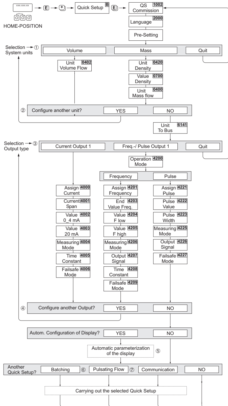
Fig. 63: Quick Setup for fast commissioning
