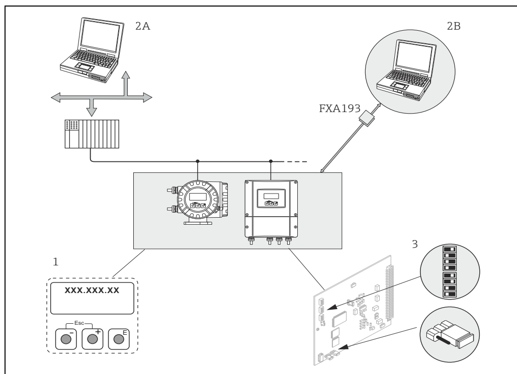
Fig. 50: Methods of operating PROFIBUS PA/DP
