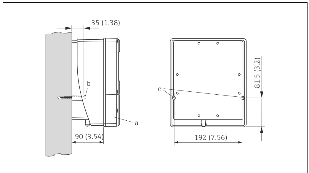
Fig. 27: Mounted directly on the wall. Engineering unit mm (inch)
