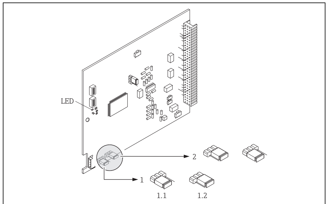
Fig. 61: Switching write protection on and off with the aid of a jumper on the I/O board
