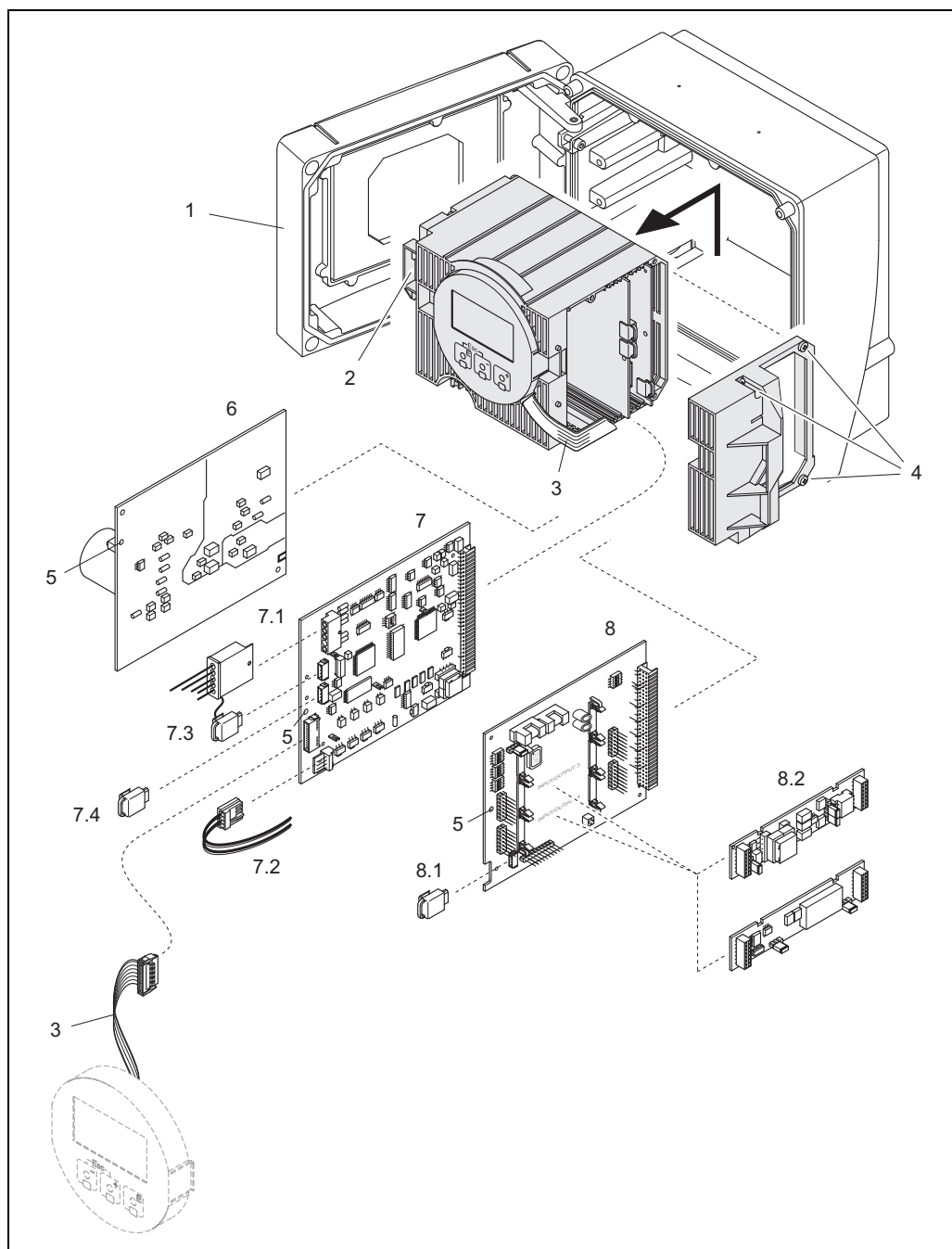
Fig. 79: Wall-mount housing: removing and installing printed circuit boards
