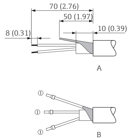
Fig. 37: Engineering unit mm (inch)
