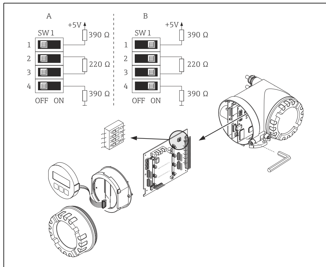
Fig. 58: Configuring the terminating resistors (for baud rates < 1.5 MBaud)
