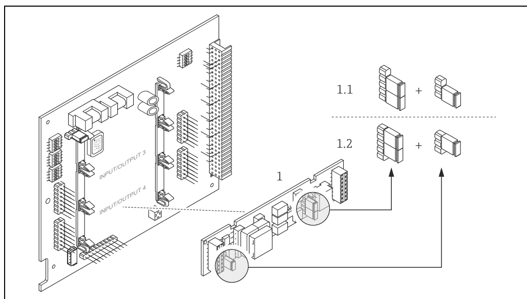
Fig. 59: Configuring the current input with the aid of jumpers (I/O board)
