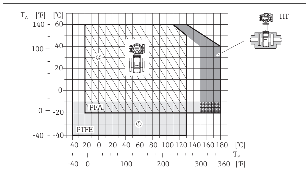
Fig. 84: Promag P compact version (with PFA or PTFE lining)
