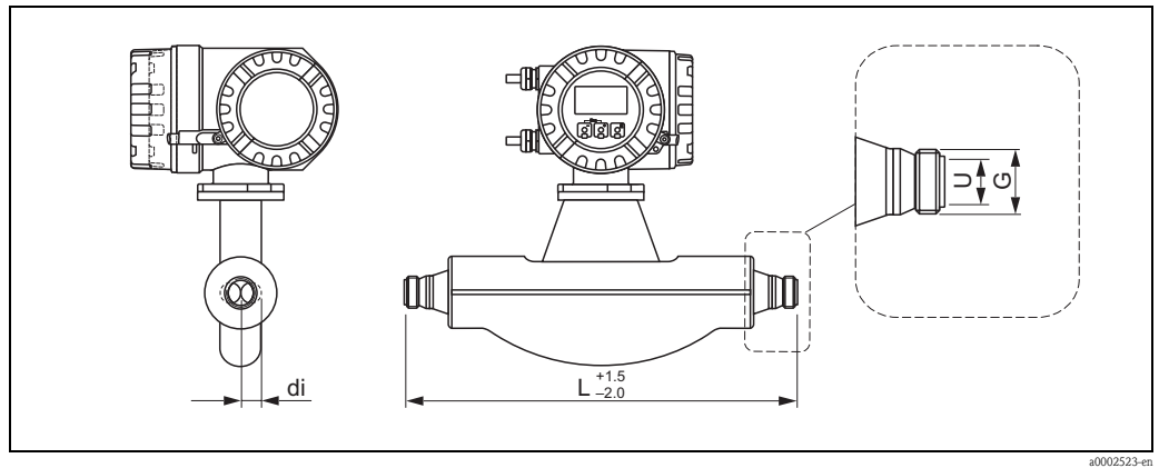
Threaded hygienic connection ISO 2853: 1.4404/316L
