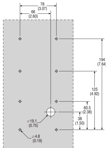
NEMA Type 4X/12 Remote (Panel Mount) HIM – Dimensions are in millimeters and (inches) Catalog Number: 22-HIM-C2
