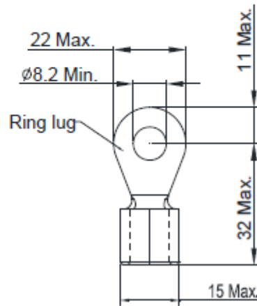
Terminal Size (Ground)
