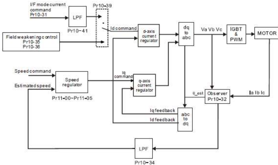
PM FOC sensorless control diagram
