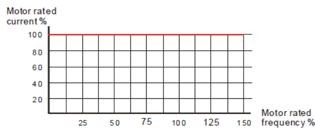
Motor cooling curve with independent fan
