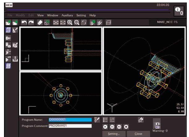
Conversational screen for lathes
