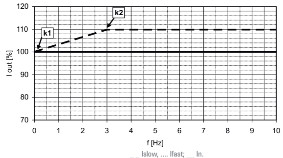
Overload LD (ADV200-...-DC-6/6A)
