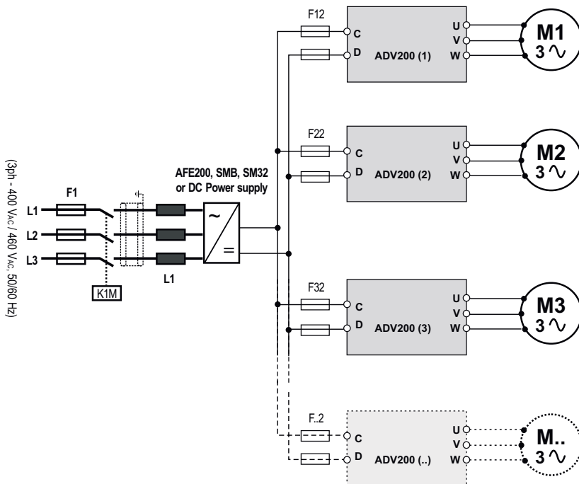
Connection of multi-drive on common DC bus with AC/DC power supply unit (with pre-load).
