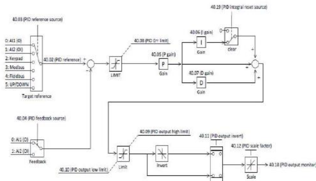
PID Control Diagram
