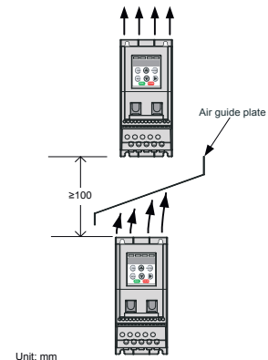
Installing one drive above another
