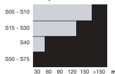
Motor wiring with unscreened cables 2-4-6 pole motors
