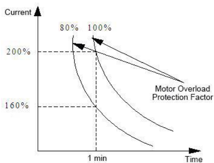
Fig.FA-1 Motor Overload Protection Factor
