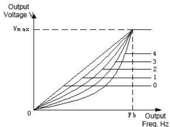
Fig. F5-1 V/F Curve
