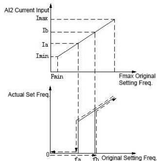
Fig. F6-1 zero-frequency function schematic diagram
