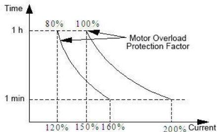
Fig. FA-2 Motor Overload Protection Factor Setting
