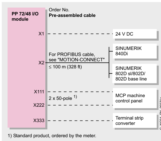
Connection overview for PP 72/48
