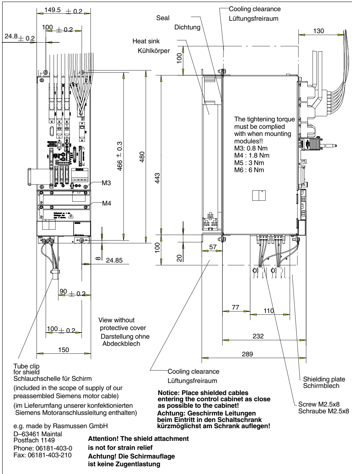
Fig. 3-5 Dimension drawing of the 2-axis CCU box
