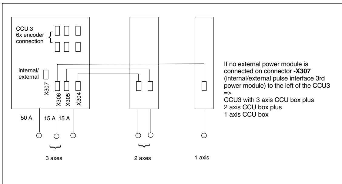
Fig. 1-4 First way of operating 6 axes on CCU3 with internal 3 axis CCU box
