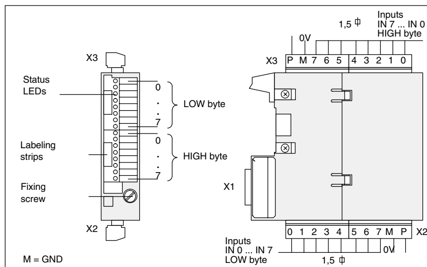
Fig. 8-1 Front view and side view of a DMP compact module 16I
