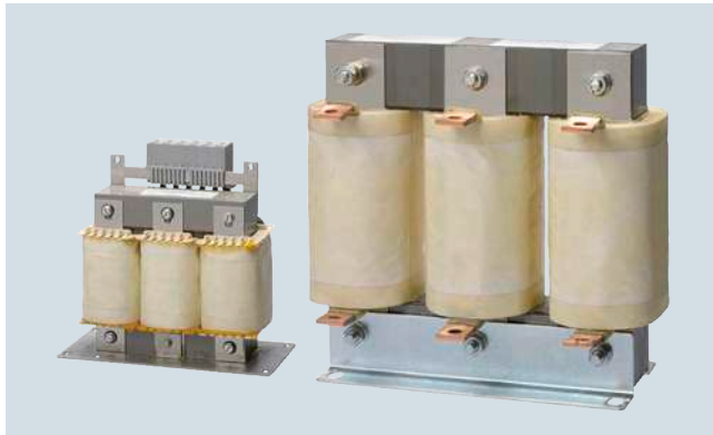
20 kW and 100 kW line reactors
