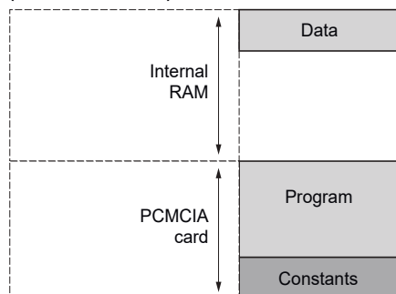
TSX 57-10 or TSX 57-20 (with PCMCIA card)
