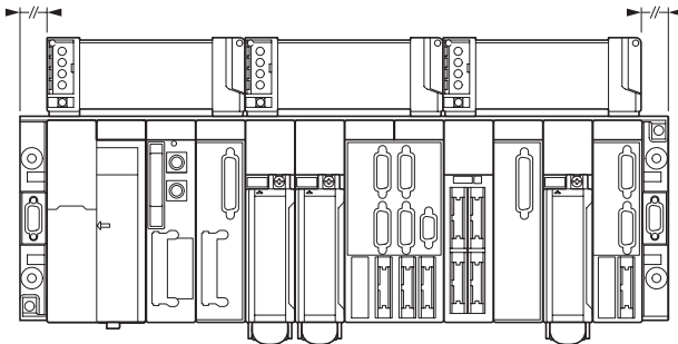
Racks with 8 positions (TSX RKY 8/8E)
