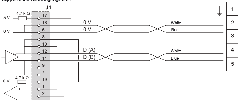
TSX SCA 50 junction box
