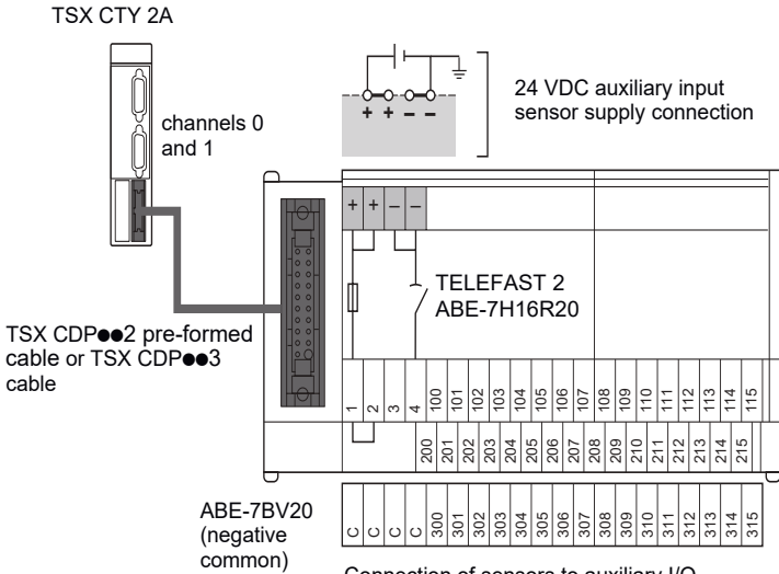
Connection of sensors to auxiliary I/O
