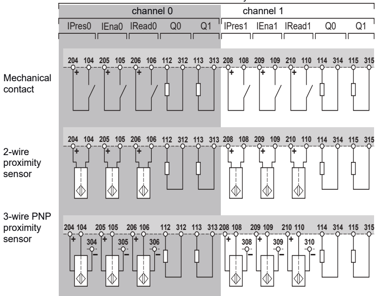
Connection of sensors to auxiliary I/O
