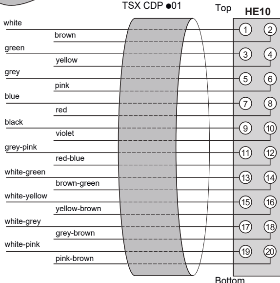
TSX CDP ●01
