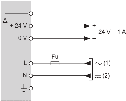
Normal connection
