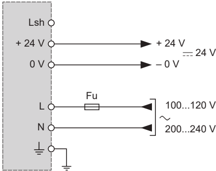
Normal connection
