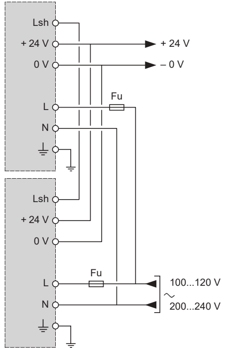
Paralleling
