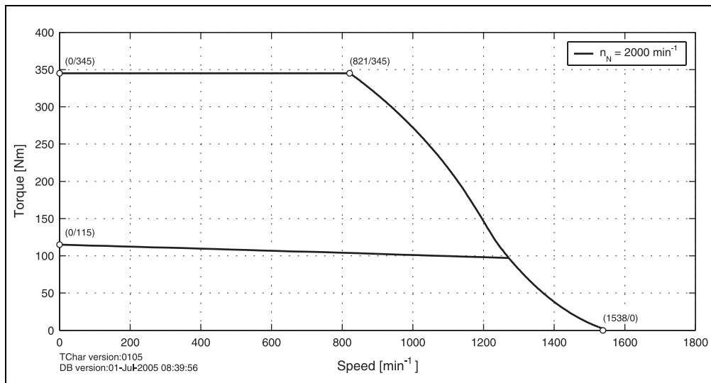
Figure 62: Speed - torque characteristic curve for 8LSA86.eennnffgg-0
