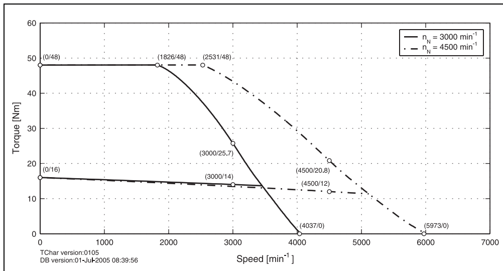
Figure 34: Speed - torque characteristic curve for 8LSA56.eennnfagg-0
