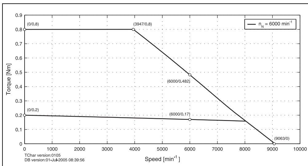
Figure 7: Speed - torque characteristic curve for 8LSA23.eennnffgg-0
