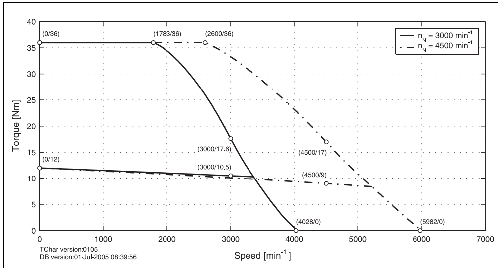
Figure 33: Speed - torque characteristic curve for 8LSA55.eennnfagg-0
