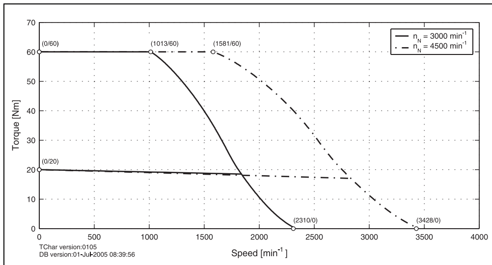
Figure 40: Speed - torque characteristic curve for 8LSA57.eennnffgg-0
