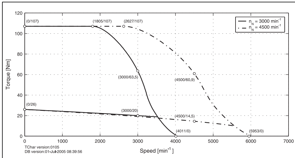
Figure 49: Speed - torque characteristic curve for 8LSA73.eennnffgg-0
