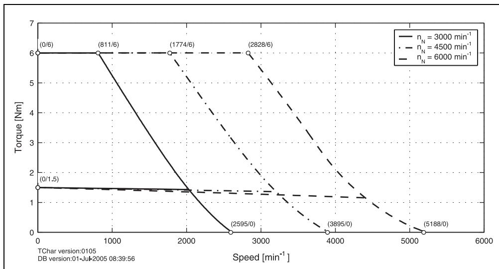
Figure 20: Speed - torque characteristic curve for 8LSA34.eennnffgg-0
