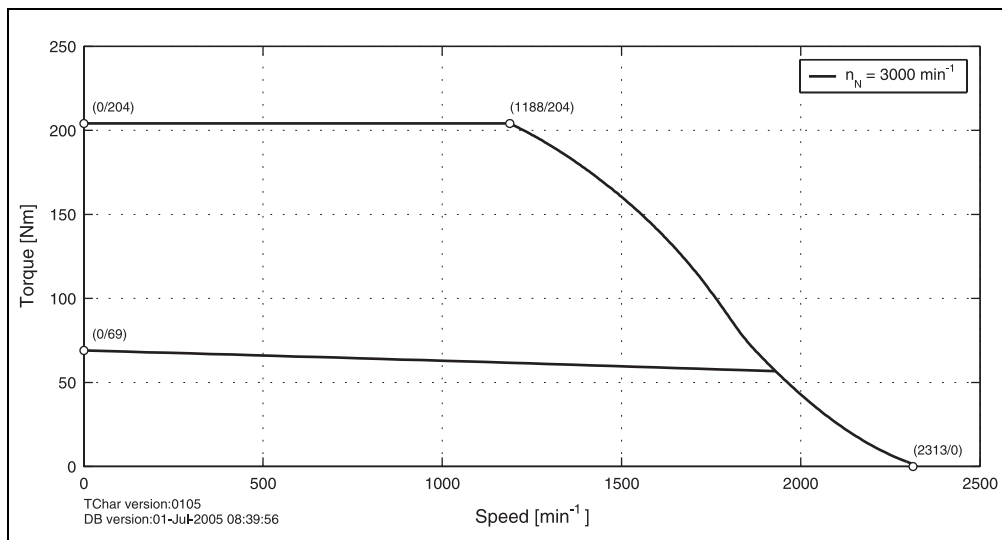
Figure 60: Speed - torque characteristic curve for 8LSA84.eennnffgg-0
