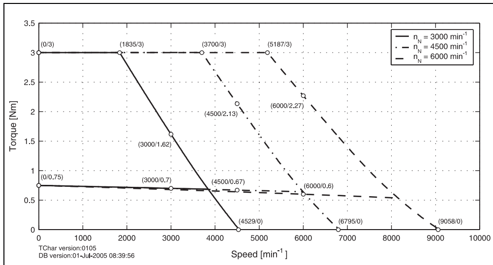
Figure 15: Speed - torque characteristic curve for 8LSA33.eennnffgg-0
