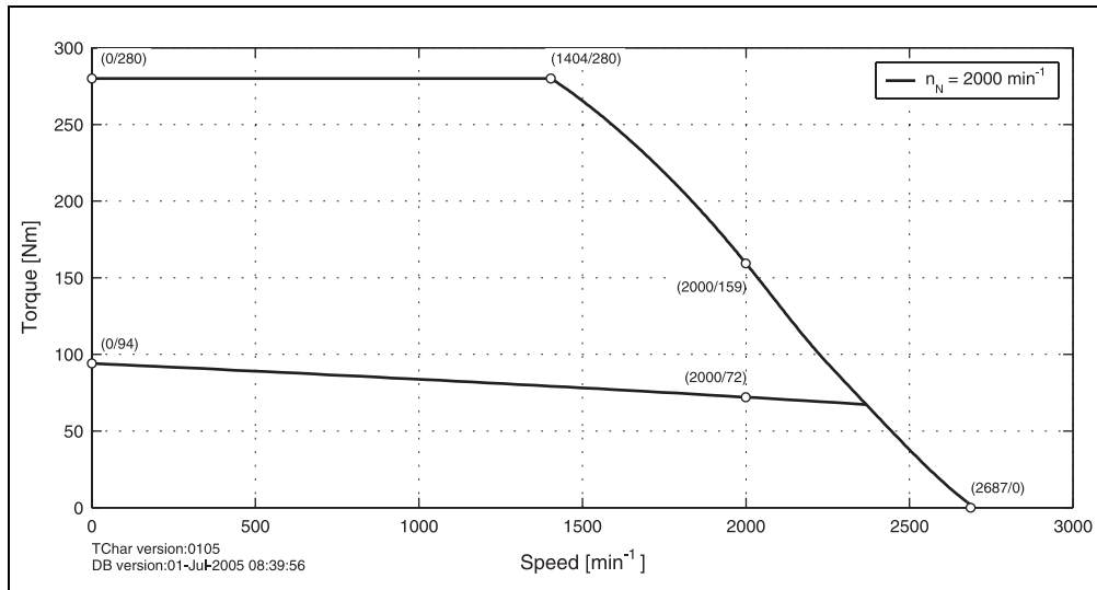
Figure 57: Speed - torque characteristic curve for 8LSA85.eennnfagg-0
