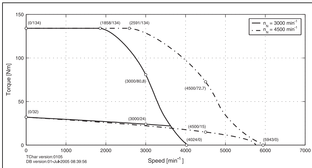
Figure 50: Speed - torque characteristic curve for 8LSA74.eennnffgg-0
