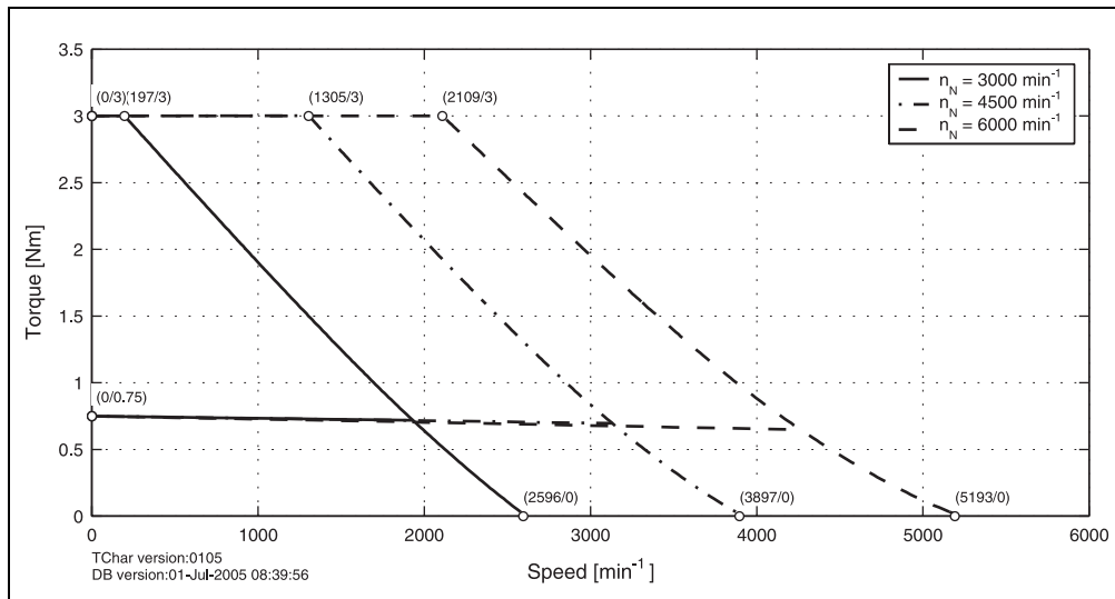
Figure 19: Speed - torque characteristic curve for 8LSA33.eennnffgg-0
