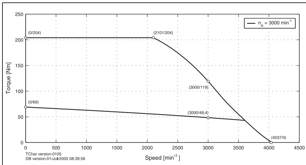
Figure 56: Speed - torque characteristic curve for 8LSA84.eennnffgg-0
