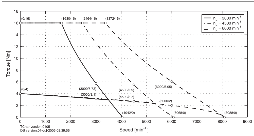
Figure 23: Speed - torque characteristic curve for 8LSA43.eennnffgg-0
