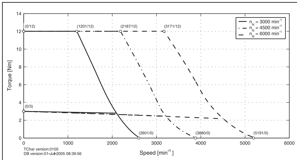
Figure 22: Speed - torque characteristic curve for 8LSA36.eennnffgg-0
