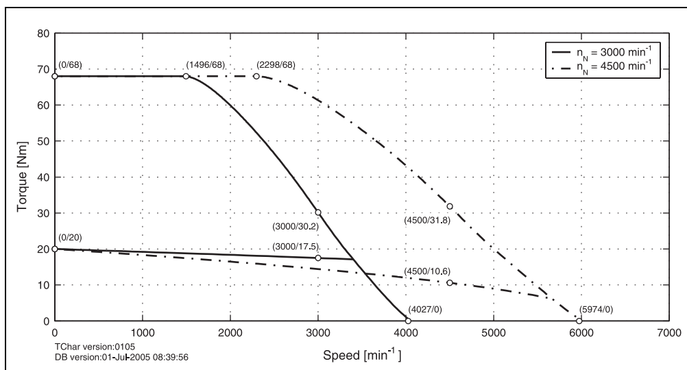
Figure 42: Speed - torque characteristic curve for 8LSA64.eennnffgg-0
