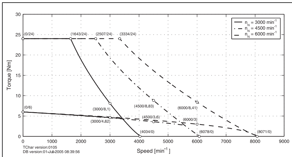
Figure 24: Speed - torque characteristic curve for 8LSA44.eennnffgg-0
