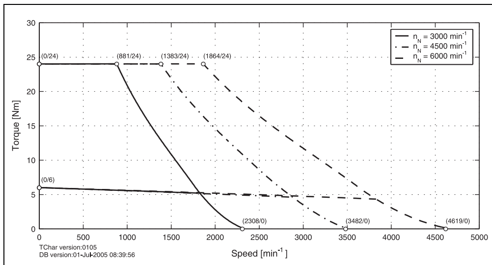
Figure 28: Speed - torque characteristic curve for 8LSA44.eennnffgg-0
