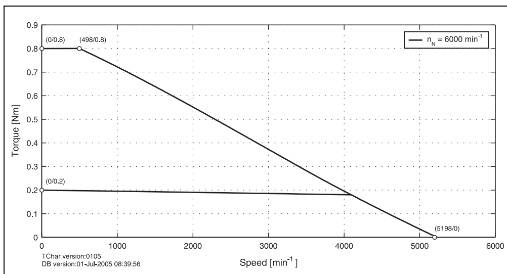
Figure 11: Speed - torque characteristic curve for 8LSA23.eennnffgg-0
