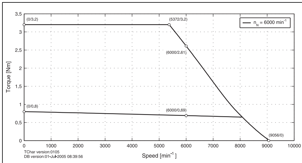
Figure 10: Speed - torque characteristic curve for 8LSA26.eennnffgg-0
