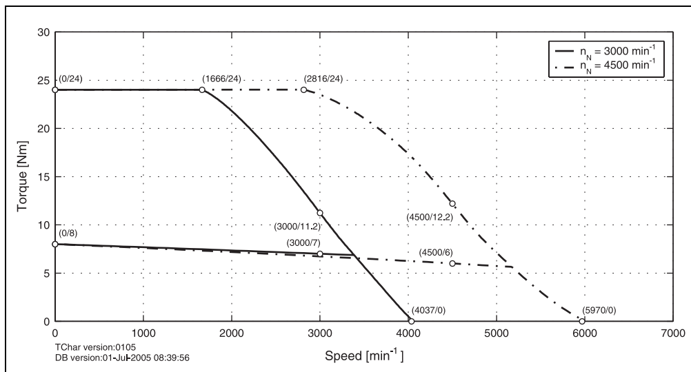
Figure 32: Speed - torque characteristic curve for 8LSA54.eennnffgg-0
