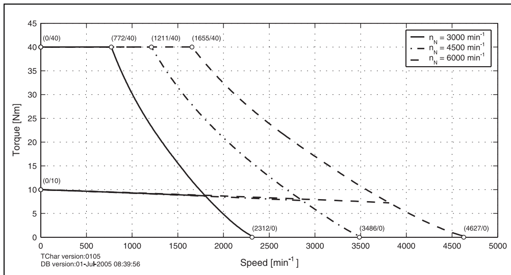
Figure 30: Speed - torque characteristic curve for 8LSA46.eennnffgg-0
