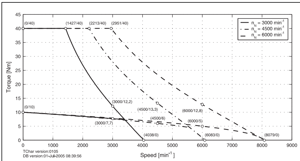
Figure 26: Speed - torque characteristic curve for 8LSA46.eennnffgg-0
