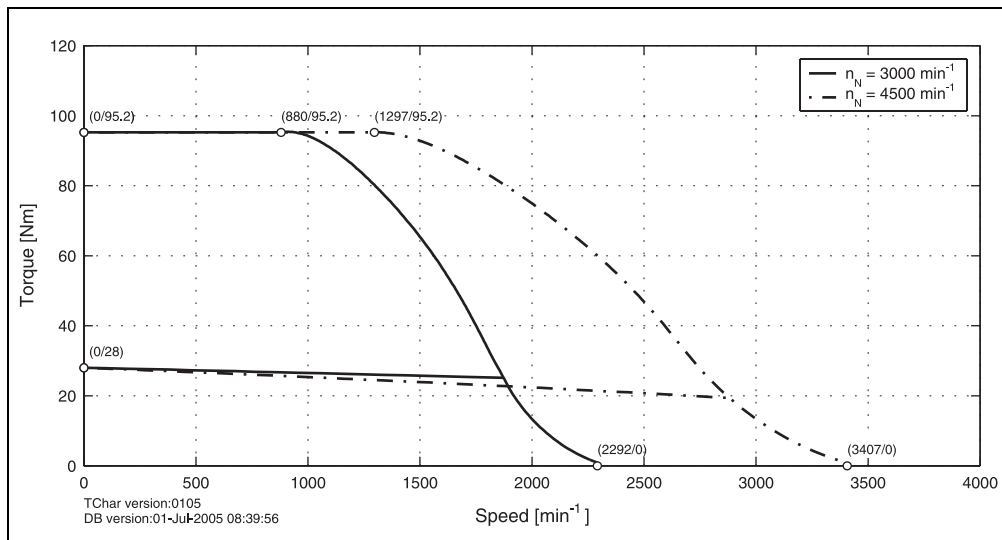
Figure 48: Speed - torque characteristic curve for 8LSA66.eennnfagg-0
