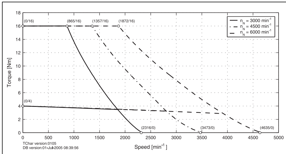
Figure 27: Speed - torque characteristic curve for 8LSA43.eennnffgg-0
