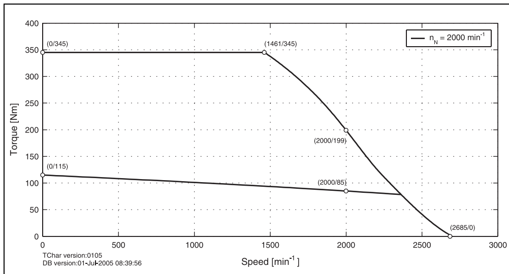
Figure 58: Speed - torque characteristic curve for 8LSA86.eennnfagg-0
