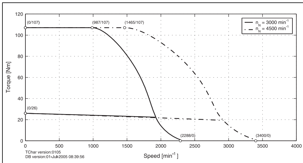
Figure 52: Speed - torque characteristic curve for 8LSA73.eennnffgg-0
