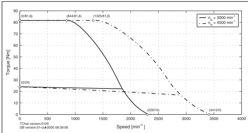
Figure 47: Speed - torque characteristic curve for 8LSA65.eennnfagg-0
