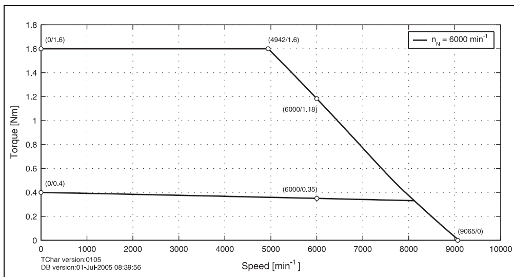
Figure 8: Speed - torque characteristic curve for 8LSA24.eennnffgg-0
