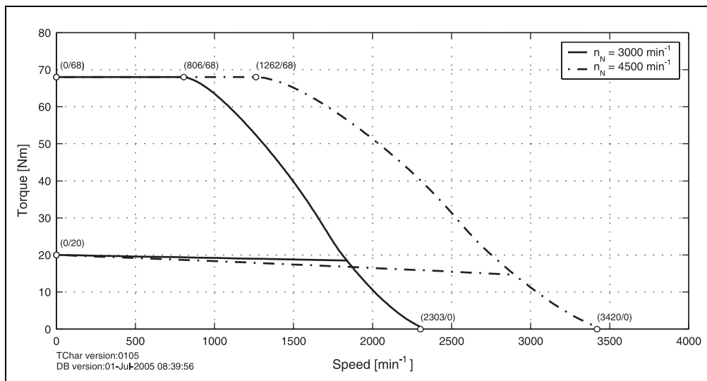
Figure 46: Speed - torque characteristic curve for 8LSA64.eennnffgg-0
