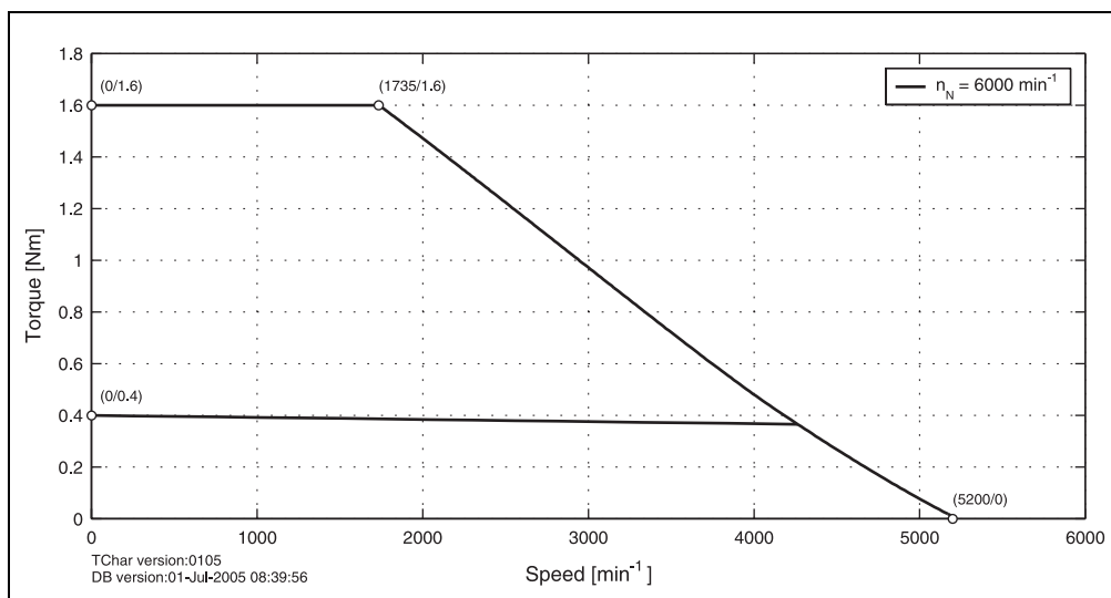
Figure 12: Speed - torque characteristic curve for 8LSA24.eennnffgg-0
