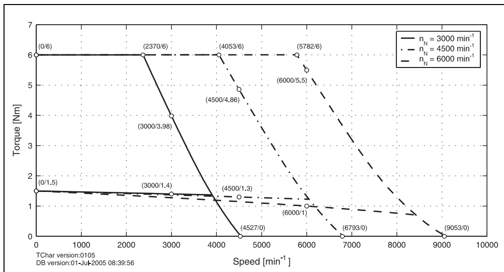
Figure 16: Speed - torque characteristic curve for 8LSA34.eennnffgg-0
