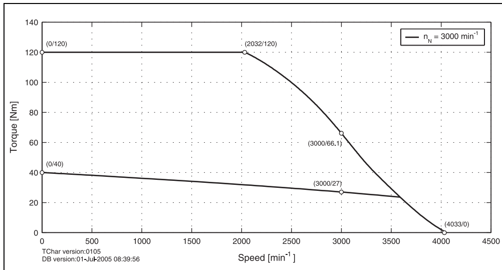
Figure 55: Speed - torque characteristic curve for 8LSA83.eennnffgg-0
