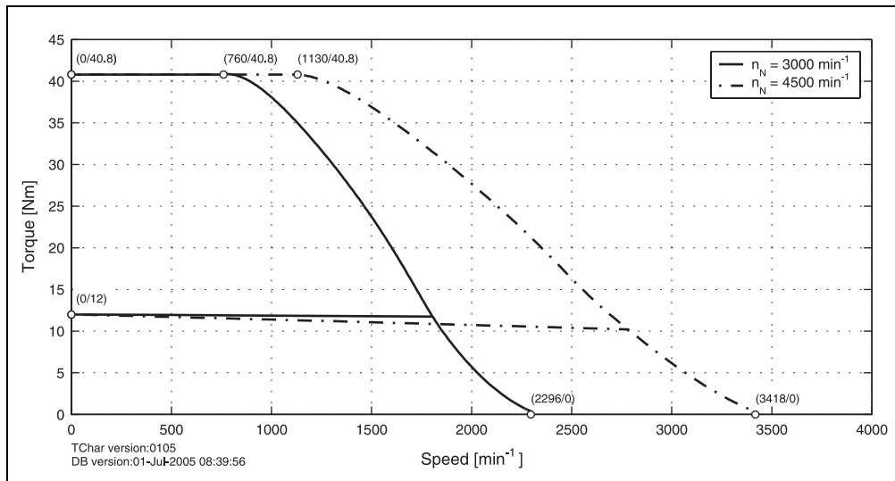
Figure 45: Speed - torque characteristic curve for 8LSA63.eennnffgg-0
