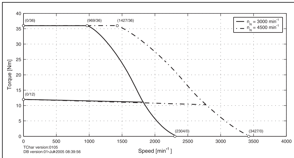
Figure 38: Speed - torque characteristic curve for 8LSA55.eennnffgg-0
