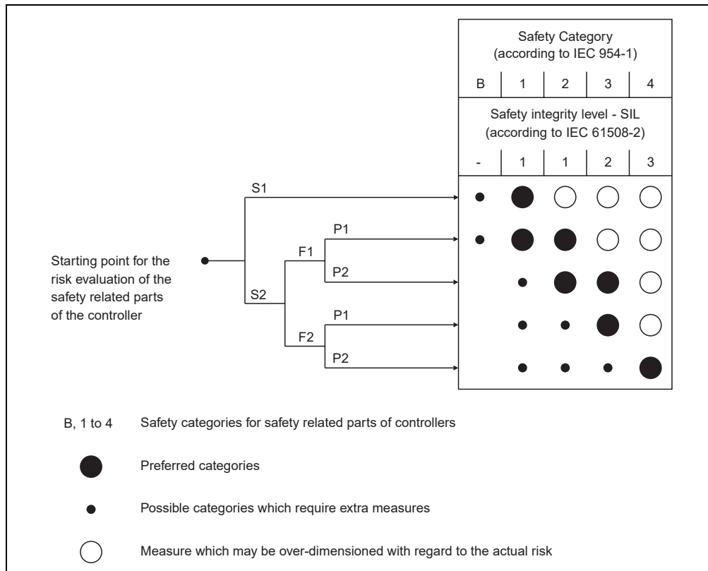
Figure 71: Risk graph according to EN 954-1, Appendix B
