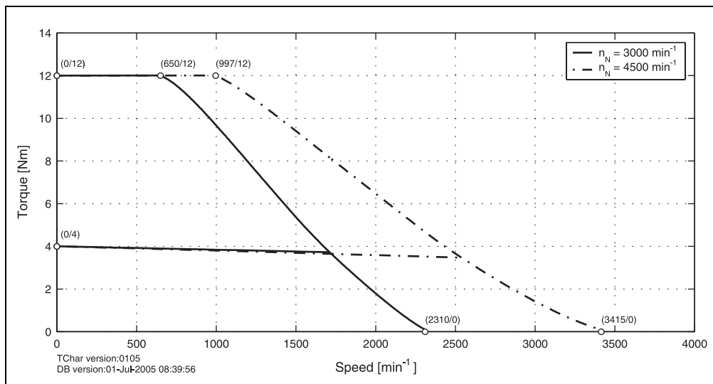
Figure 36: Speed - torque characteristic curve for 8LSA53.eennnffgg-0
