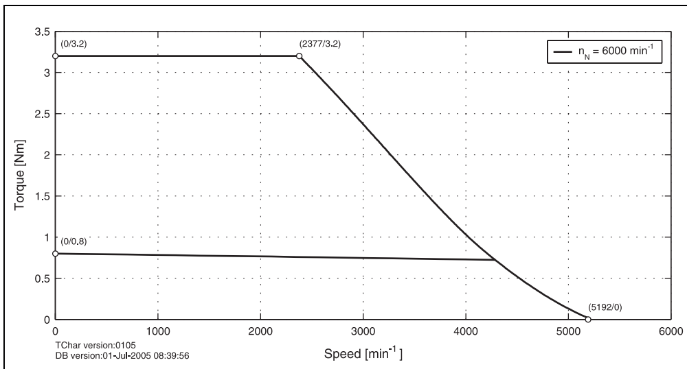
Figure 14: Speed - torque characteristic curve for 8LSA26.eennnffgg-0
