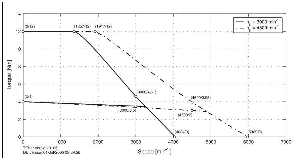
Figure 31: Speed - torque characteristic curve for 8LSA53.eennnffgg-0
