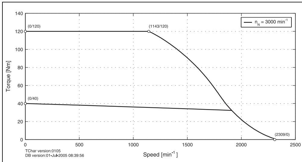
Figure 59: Speed - torque characteristic curve for 8LSA83.eennnffgg-0
