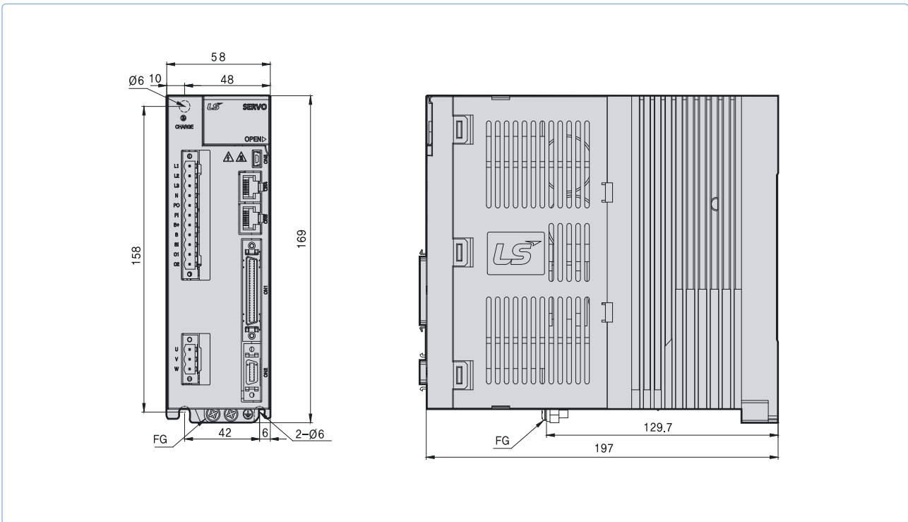
XDL-L7SA008 □ ~ XDL-L7SA010 □ [Weight : 1.5kg(Fan-Cooling included)]
