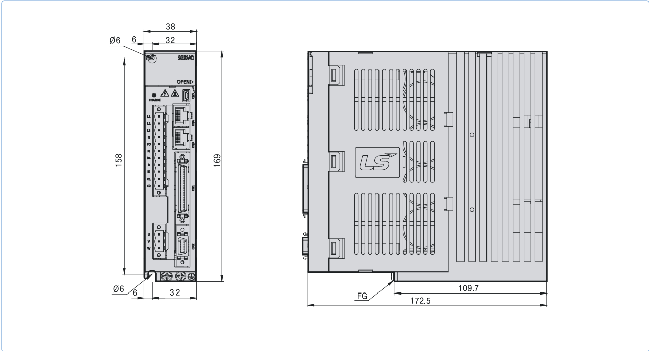
XDL-L7SA001 □ ~ XDL-L7SA004 □ [Weight 1.2kg]
