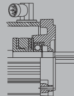
Holding brake
