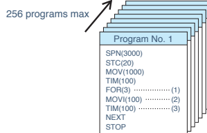
Program example
