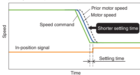
[Settling time comparison with the prior model]
