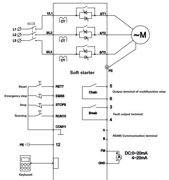
Wiring diagram
