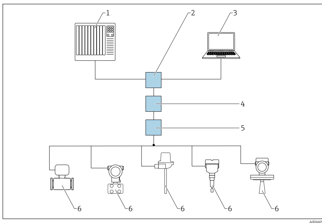
12 Options for remote operation via PROFINET over Ethernet-APL network: star topology
