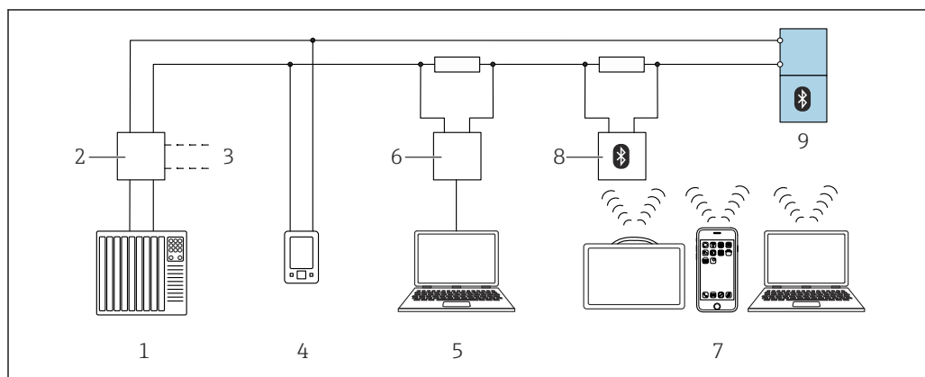
9 Options for remote operation via HART protocol
