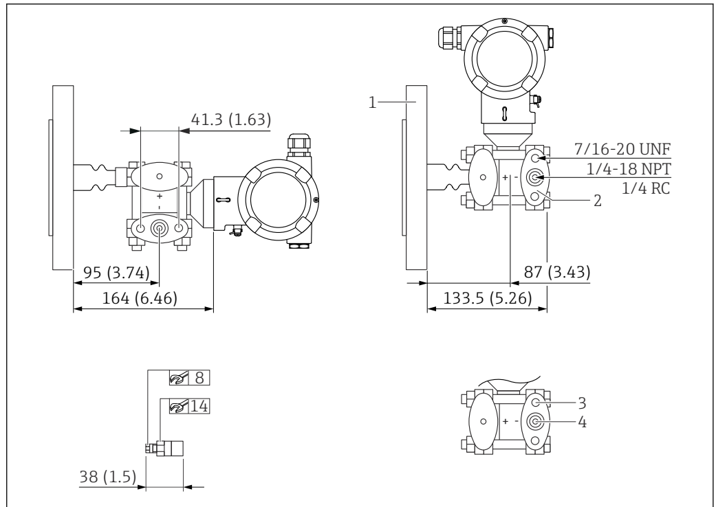
Device with short temperature isolator
